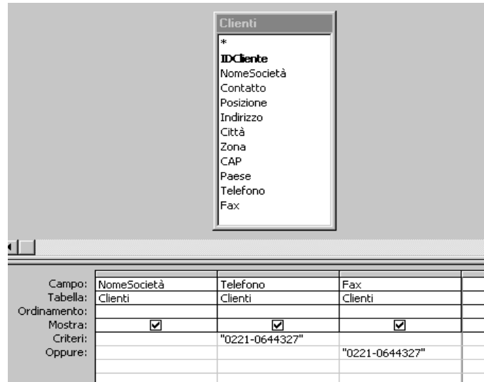
Access - Query
