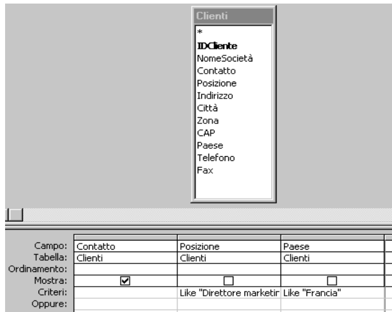
Access - Query
