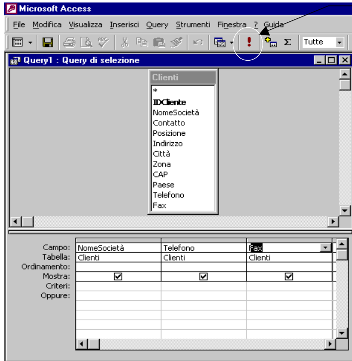
Access - Query
